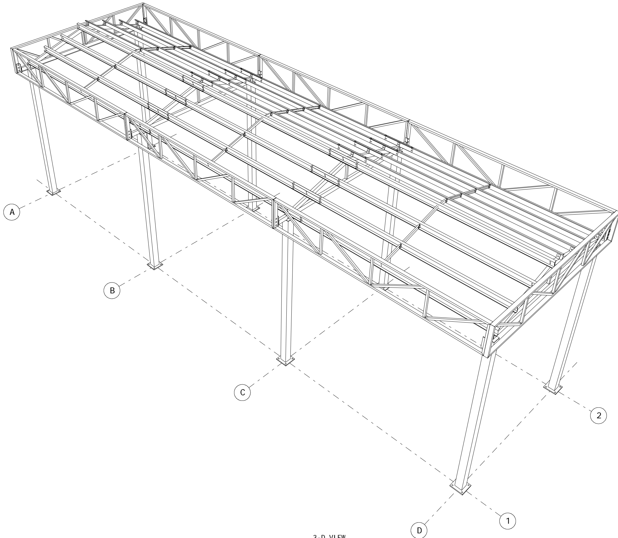
3-D VIEW
